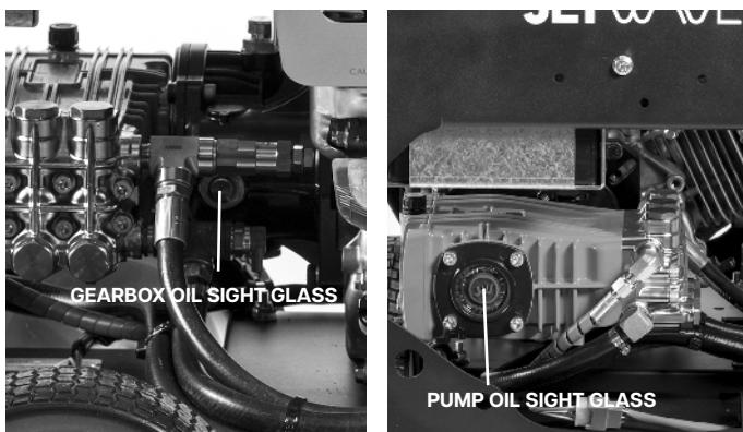
Figure.10 - Checking Pump and Gearbox Oil Level
